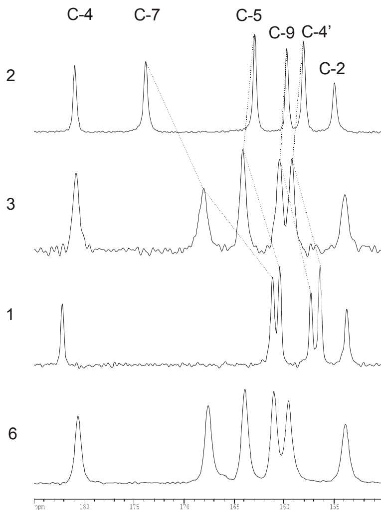
Fig. 1S Comparison of ^{13}\text{C} solid state NMR spectra (expanded region) of 1 - 3 . The spectrum of 6 is shown for comparison. The assignments for 6 are as in 3 except that 9 and 4' are interchanged.
